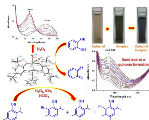
Functional mimics of vanadium haloperoxidase and catechol-oxidase
