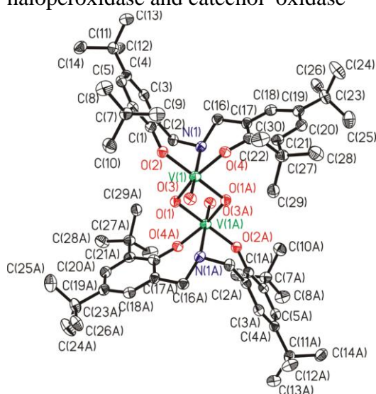
\mu -Bis(hydroxidobis{oxidovanadium(V)}) complex
