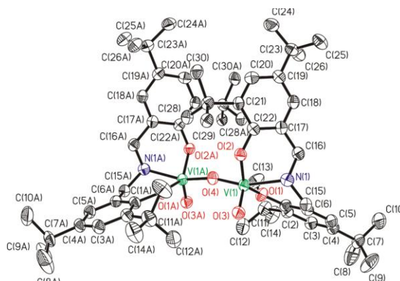
\mu -Oxidobis{oxidovanadium(V)} complex
